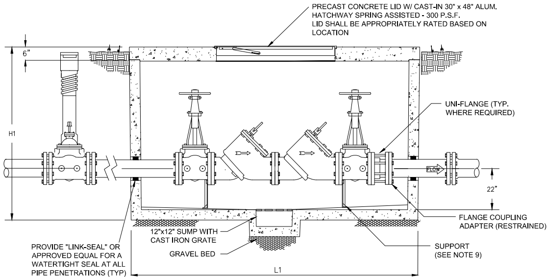
ELEVATION NTS
